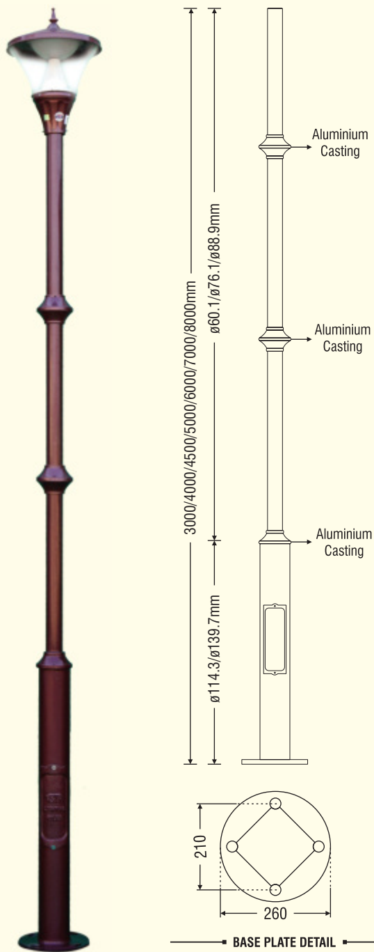
BASE PLATE DETAIL Upto 5 Mtr. - 12mm, Above 6 Mtr. - 16mm Thk.
